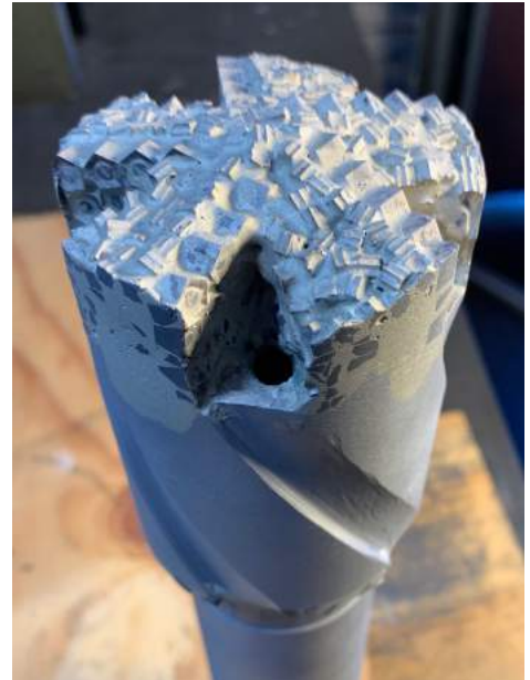
Options shown above are Closed Center Patriot 5 Sided Inserts backed with Starbide and with extended reverse spiral gage.
